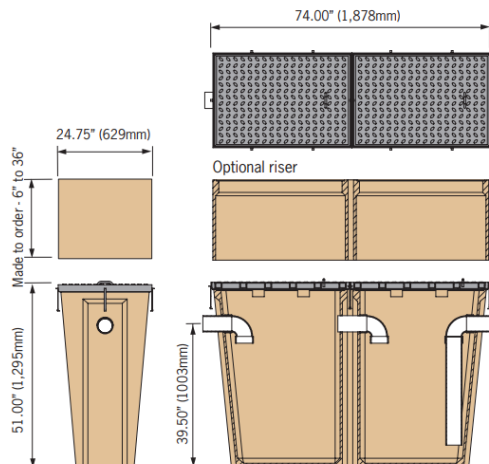
Separator with frame & heavy duty cover
