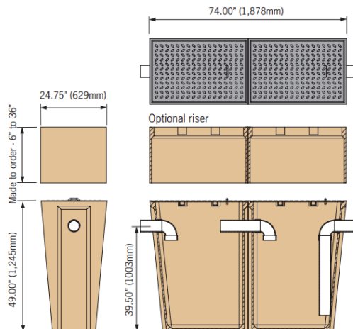
Separator with light duty cover
